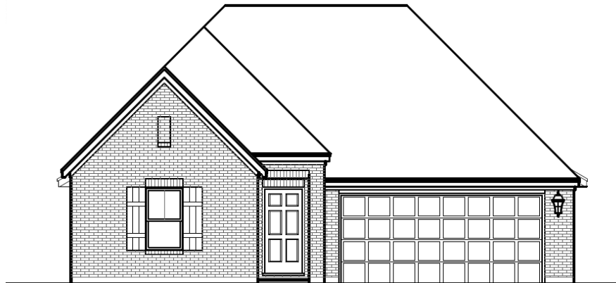
ELEVATION F
