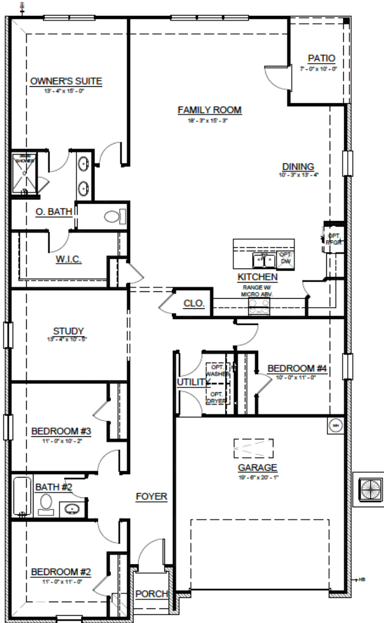
MAIN FLOOR - ELEVATION D
