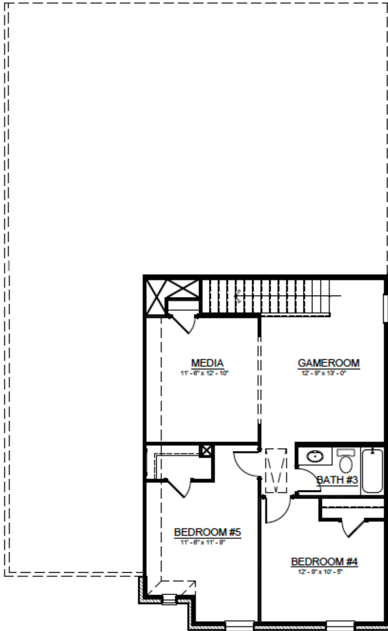
UPPER FLOOR - ELEVATION D
