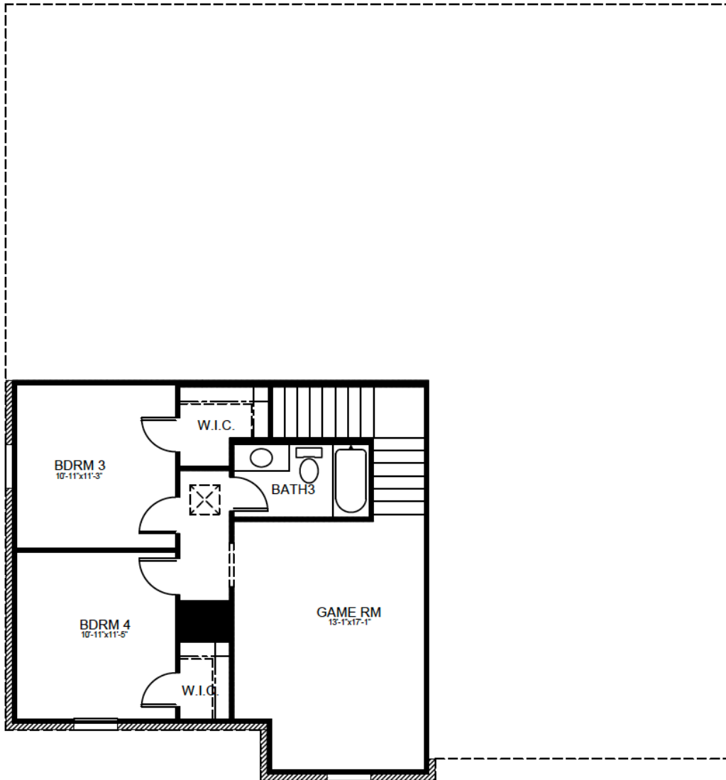
UPPER FLOOR - ELEVATION D
