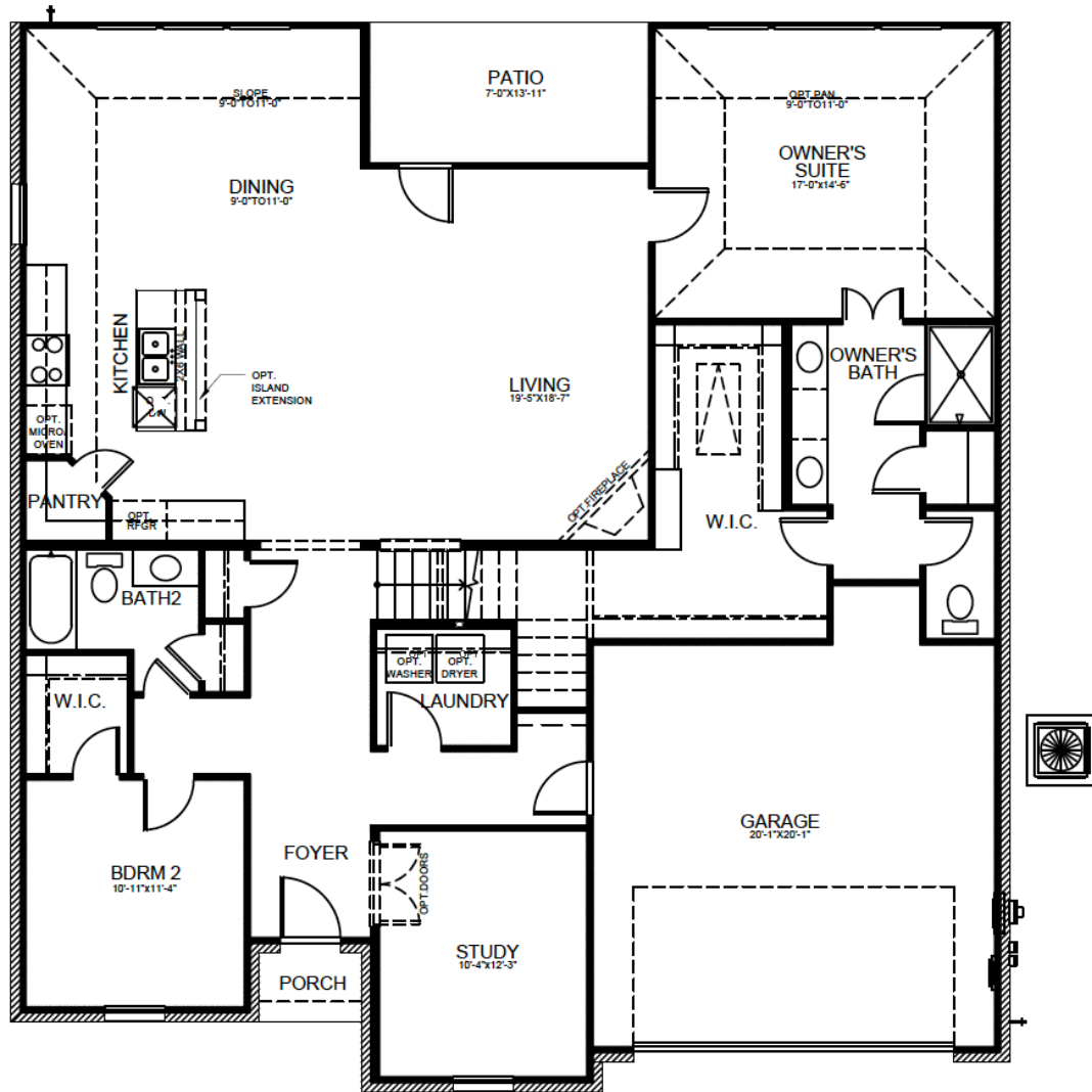
MAIN FLOOR - ELEVATION D
