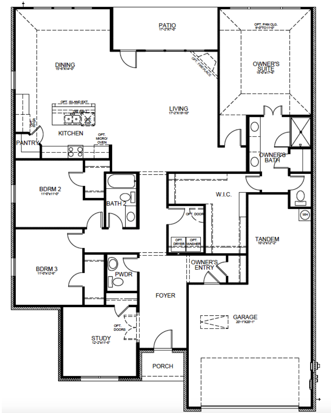
MAIN FLOOR - ELEVATION D
